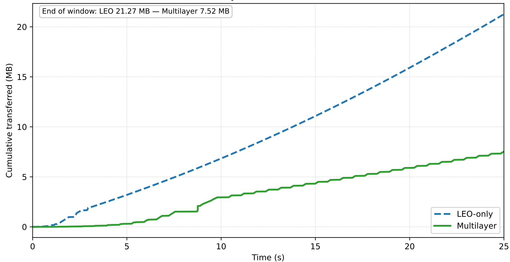
Figure K — Cumulative bytes vs time — 25 s sim, 1000 ms state updates Tokyo to Buenos-Aires
